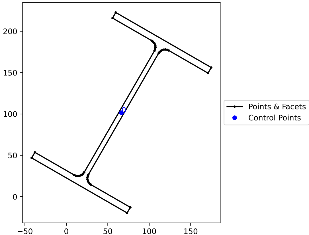
Cross-Section Geometry
