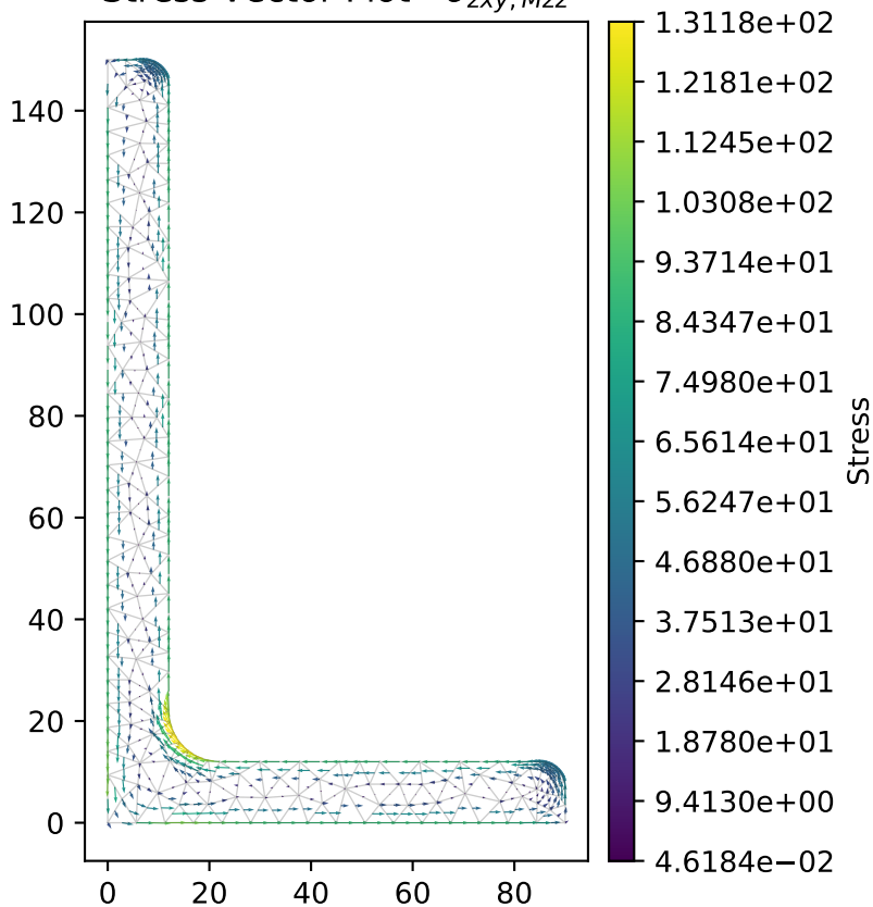
Stress Vector Plot - \sigma_{zxy, Mzz}
