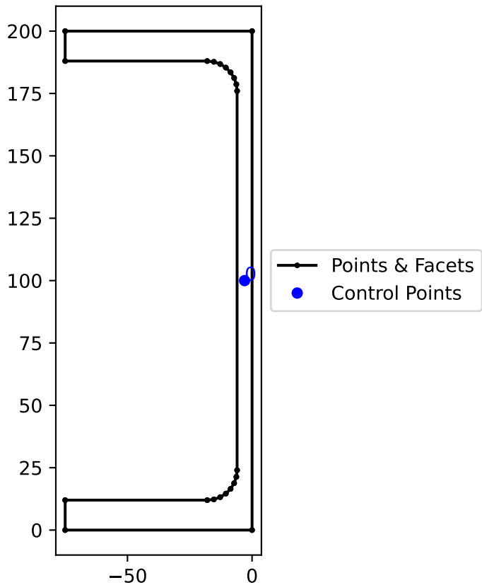
Cross-Section Geometry
