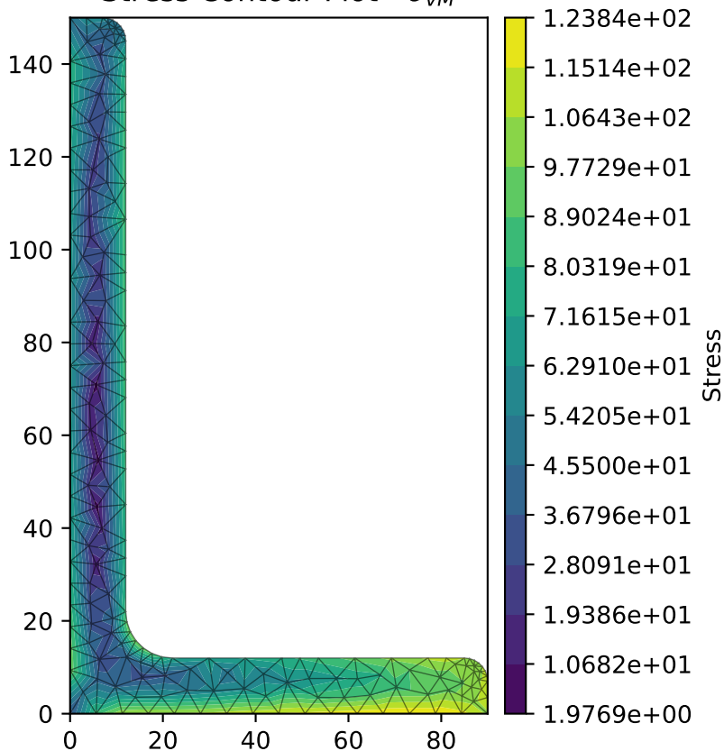
Stress Contour Plot - \sigma_{VM}
