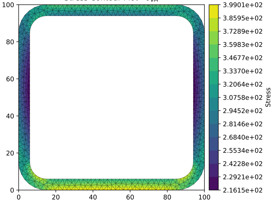
Stress Contour Plot - \sigma_{VM}
