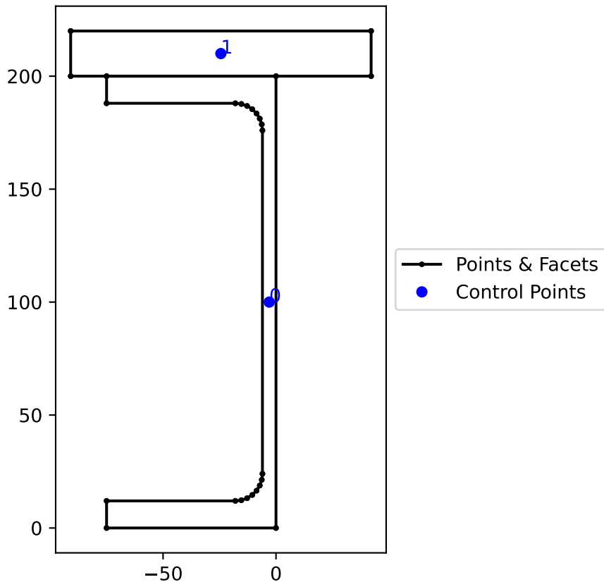
Cross-Section Geometry
