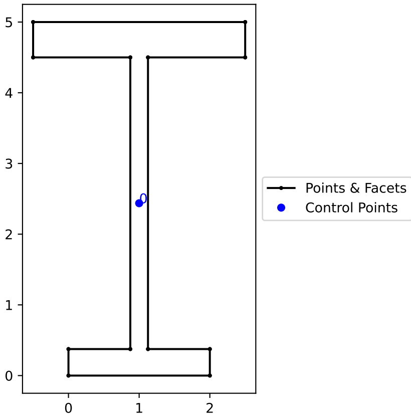
Cross-Section Geometry
