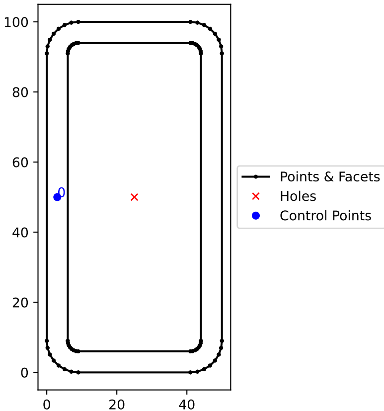
Cross-Section Geometry
