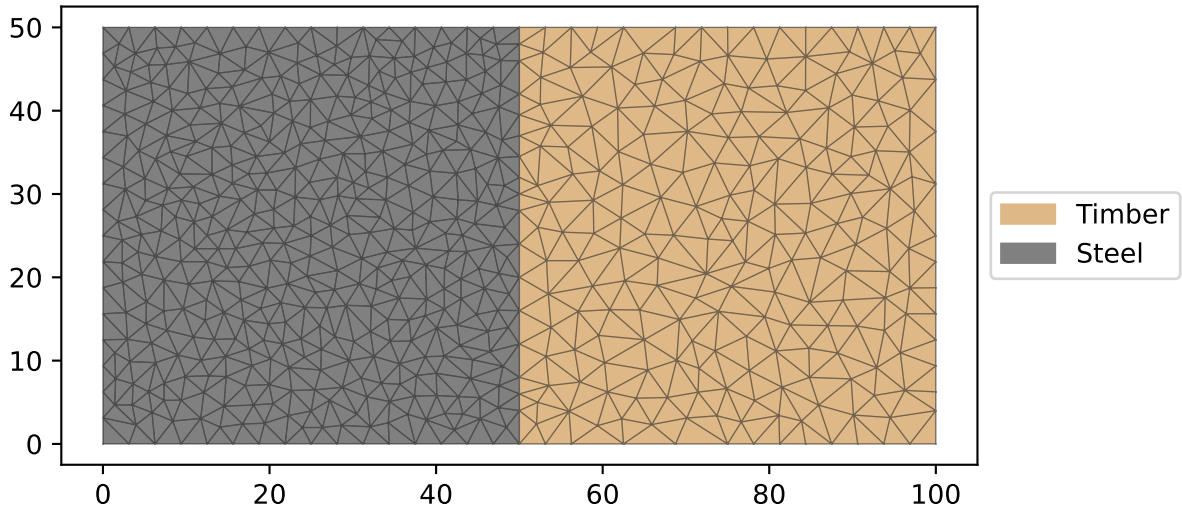
Finite Element Mesh
