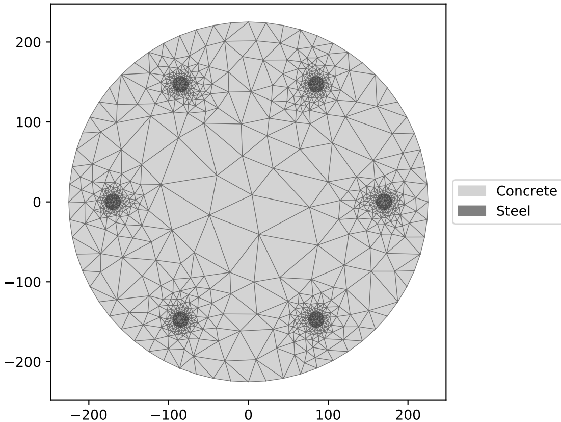
Finite Element Mesh
