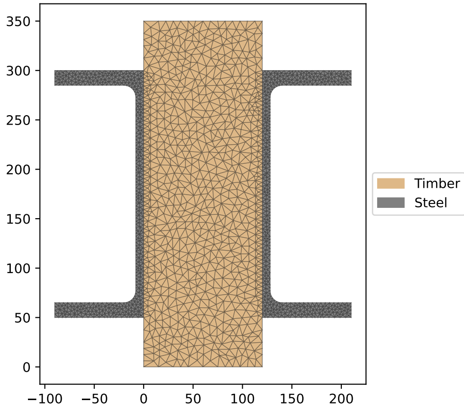
Finite Element Mesh
