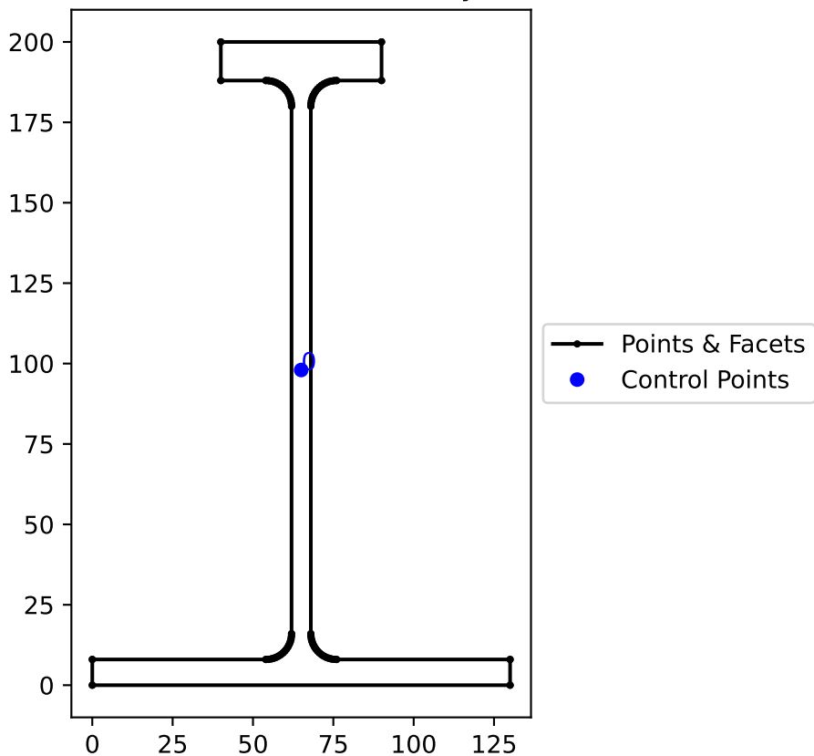
Cross-Section Geometry
