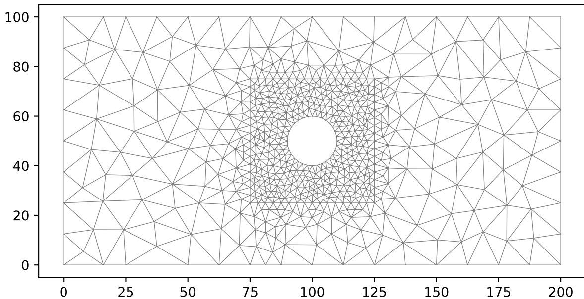
Finite Element Mesh
