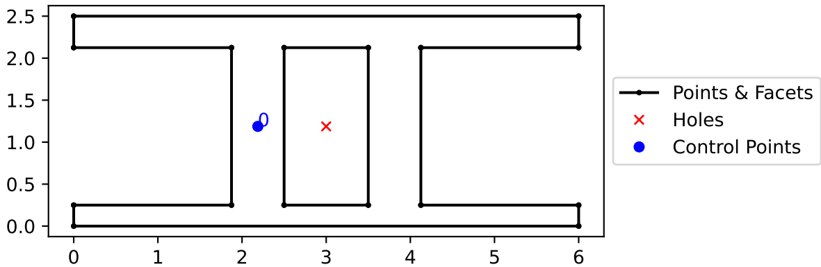
Cross-Section Geometry
