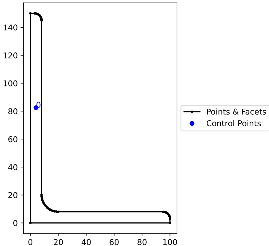
Cross-Section Geometry
