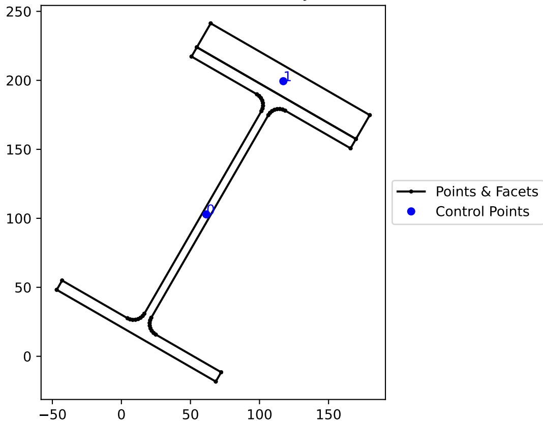
Cross-Section Geometry
