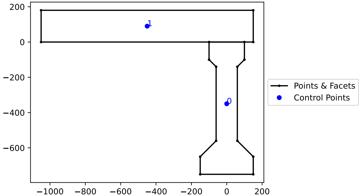
Cross-Section Geometry
