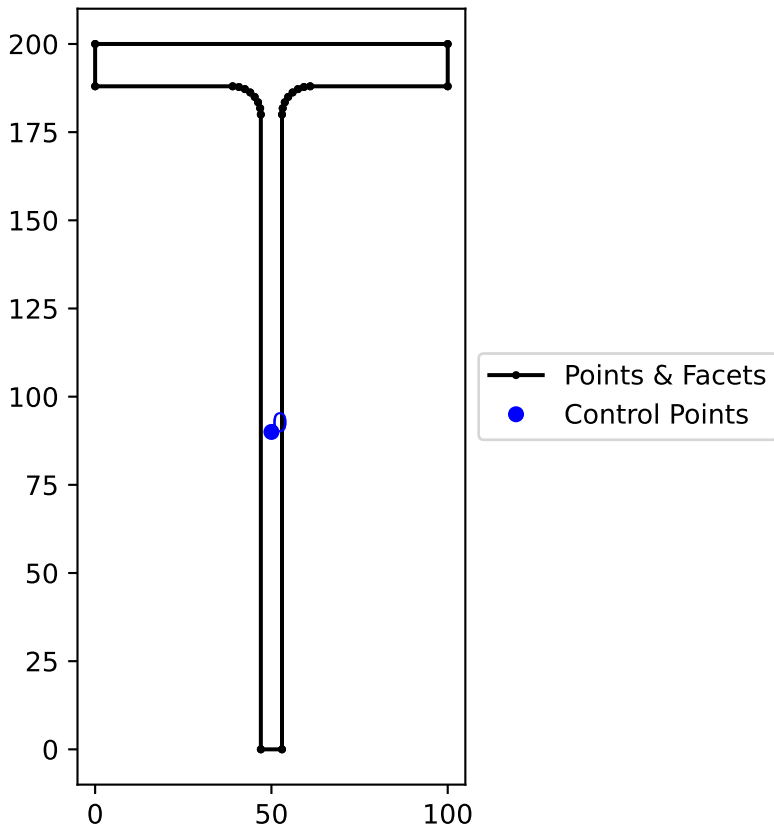
Cross-Section Geometry
