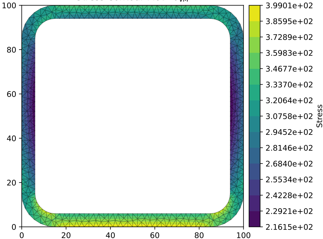
Stress Contour Plot - \sigma_{VM}
