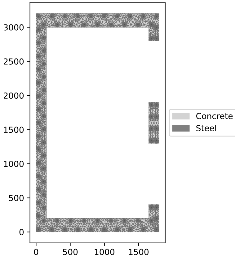
Finite Element Mesh
