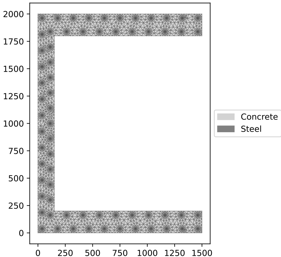
Finite Element Mesh
